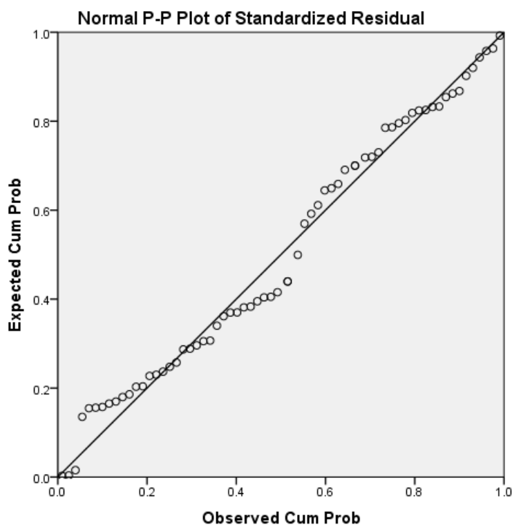
Figure 9: probability plot diagram for normality of the dependent variable (project performance).
