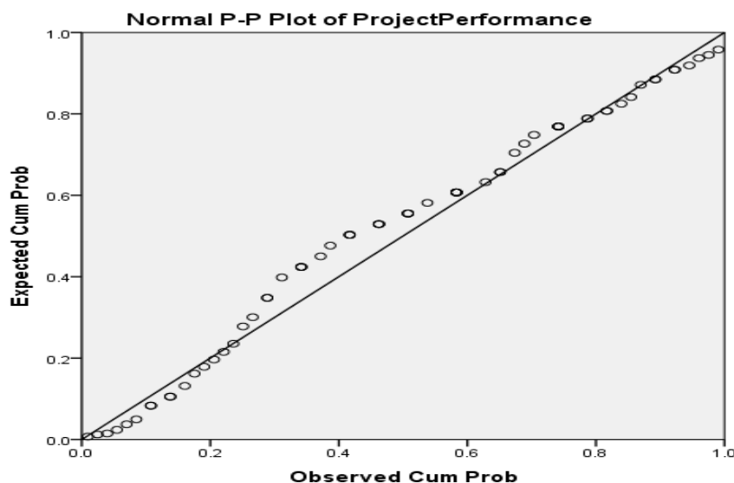
Figure 5: Probability plot diagram for linearity of the dependent variable (project performance).
